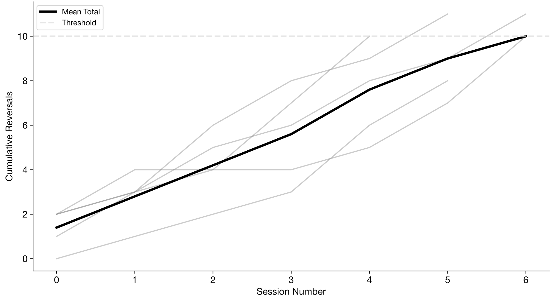
Cumulative Total Reversals Over Time (n=5 subjects; sessions per subject=5-7)
